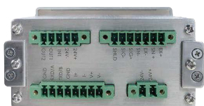
RS485/232 + Analog output
