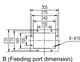
B (Feeding port dimension)
