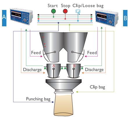
Double Channel Packaging Controller with Hopper
