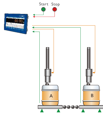
Double Nozzle for Liquid Filling Application
