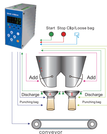
Duplex Packing Controller without Hopper
