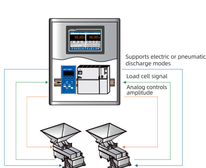
GMC-X802CD for 2 Linear Feeder Packing Machine without PLC
