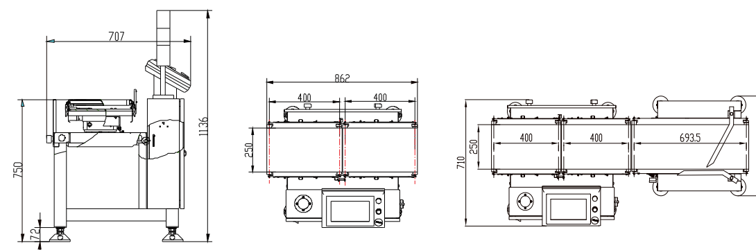
Low Cabinet
