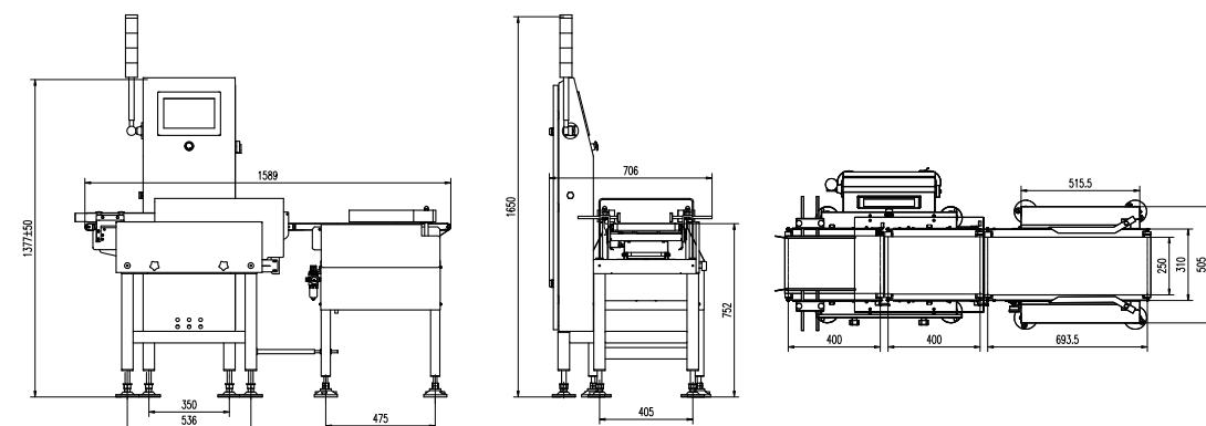
High Cabinet
