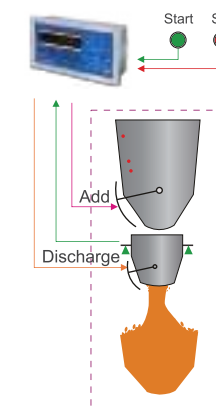
Continuous Weighing
