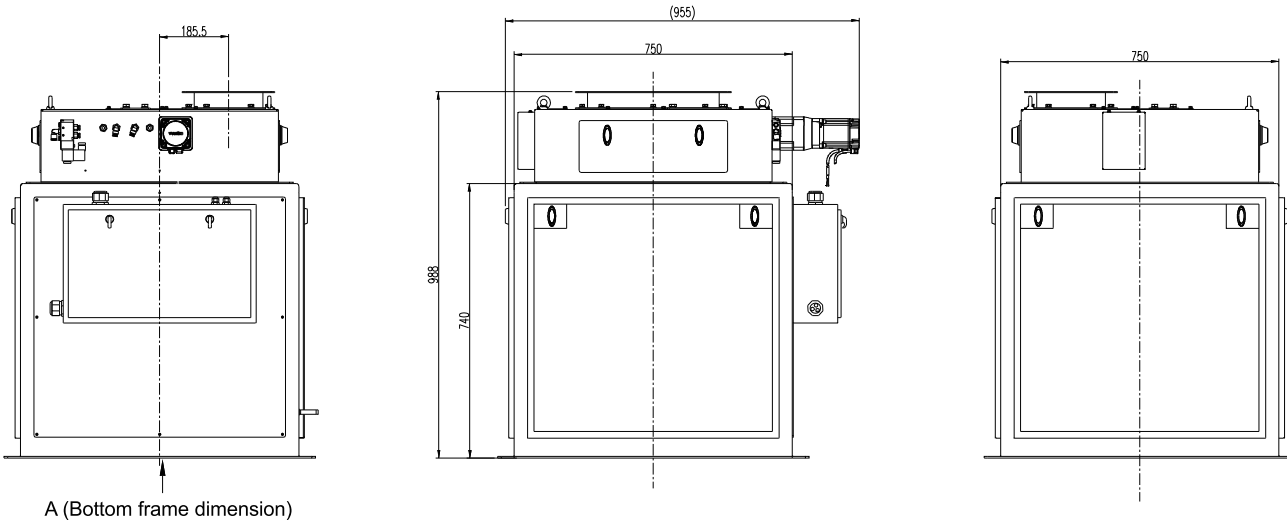
A (Bottom frame dimension)
